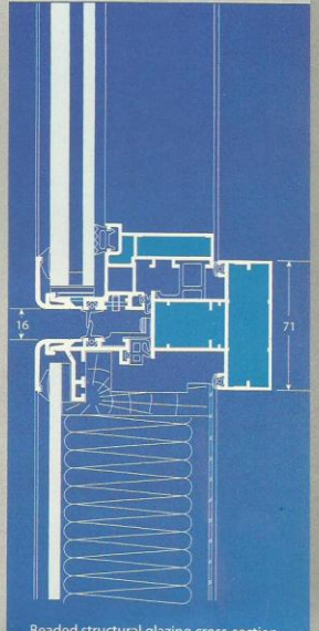
Beaded structural glazing cross-section
