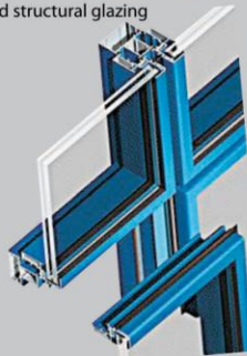
Glazing, gaskets and beads are clipped
